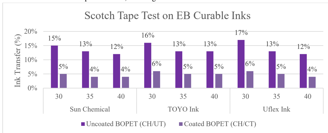
Fig. 1, Comparative Analysis of Ink Adhesion Test On Curable Inks
