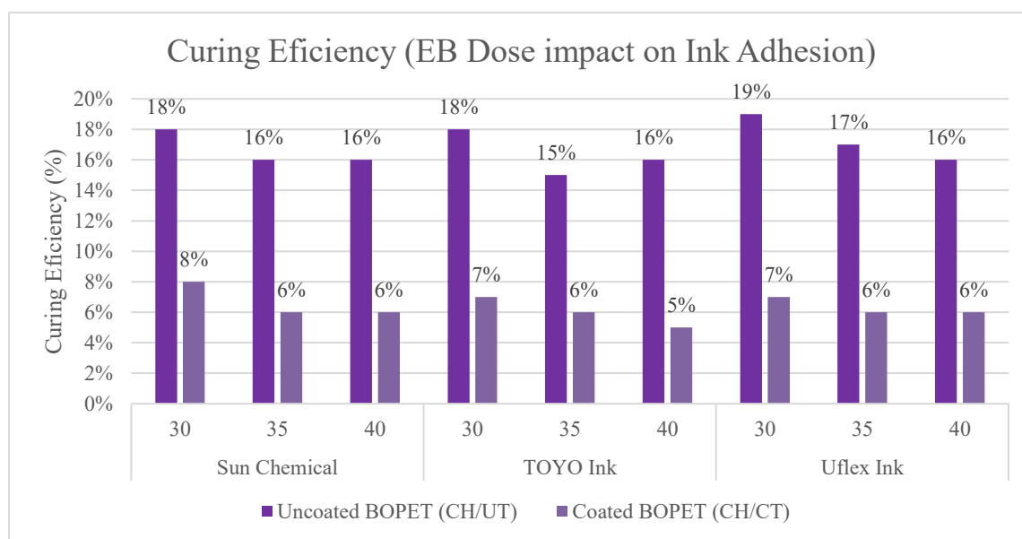
Fig. 2, Comparative Analysis of Surface Energy Test on Curable Inks
