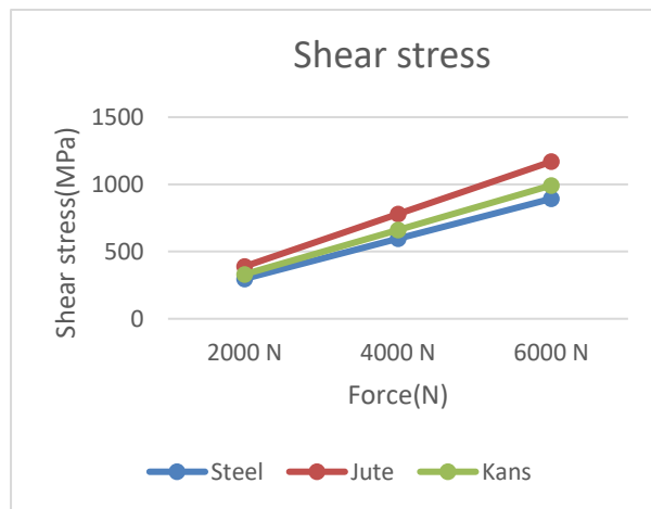
Figure 6: Shear stress with respect to force (N)
