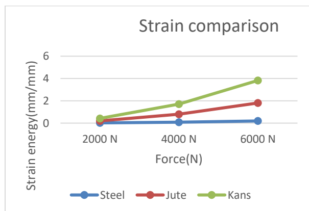
Figure 8: Strain energy with respect to force (N)
