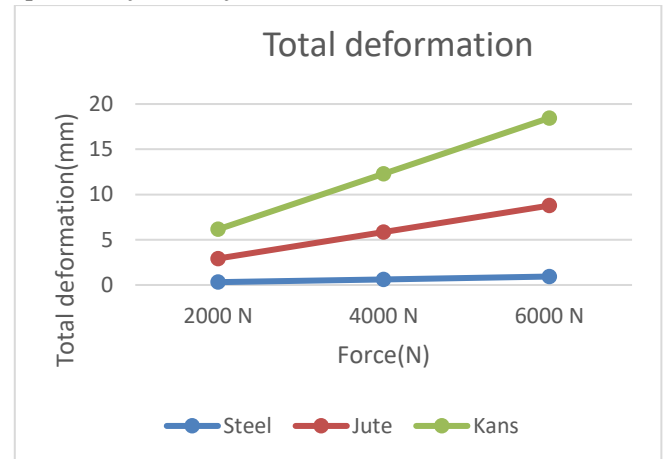
Figure 9: Total deformation with respect to force (N)
