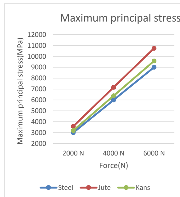
Figure 5: Maximum principal stress with respect to force (N)
