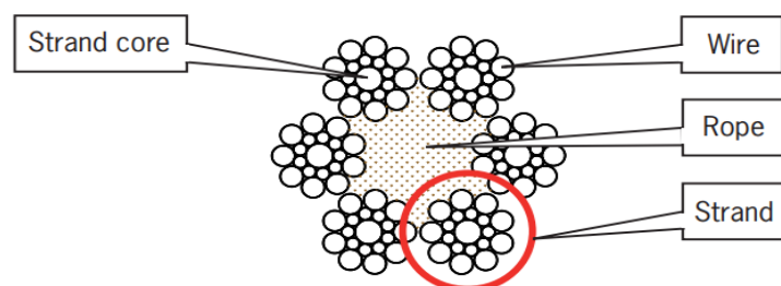
Figure 1: Cross section of a steel wire rope with the components of the rope clearly indicated
