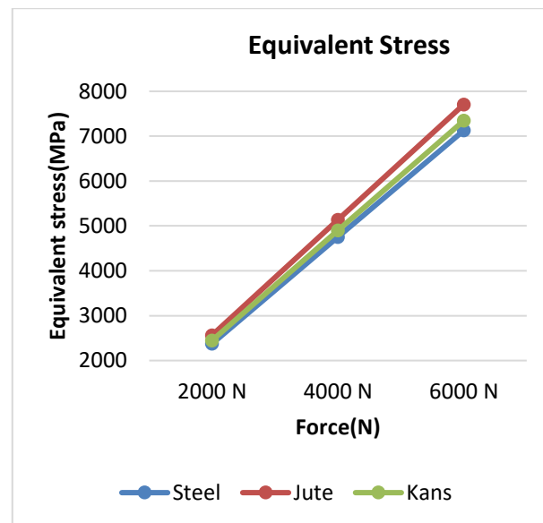
Figure 4: Equivalent stress with respect to force (N)
